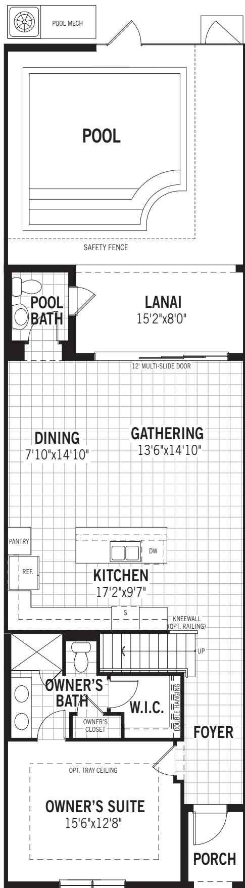
FIRST FLOOR
